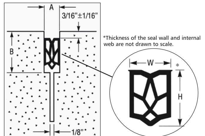
Typical joint design for the "E" and "V" series pavement seals
