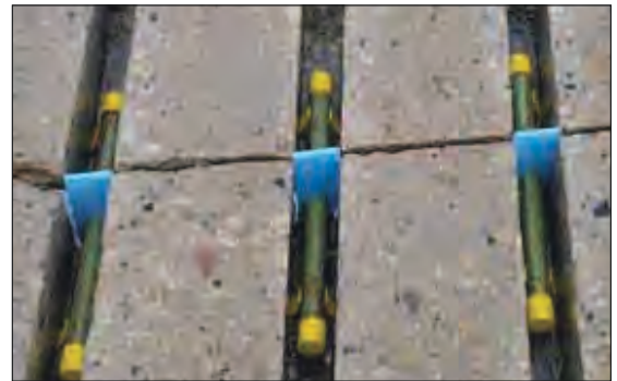
Placing the dowel bars, caps, chairs and joint filler.
