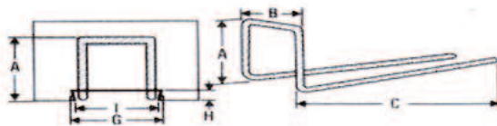
STABOX TYPE 160D (No. 4 or 5 rebar)
