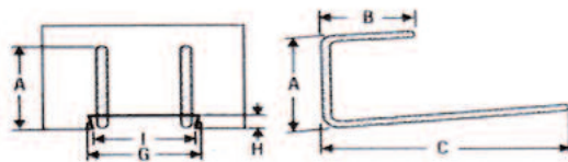
STABOX TYPE 160DD (No. 4 or 5 rebar)
